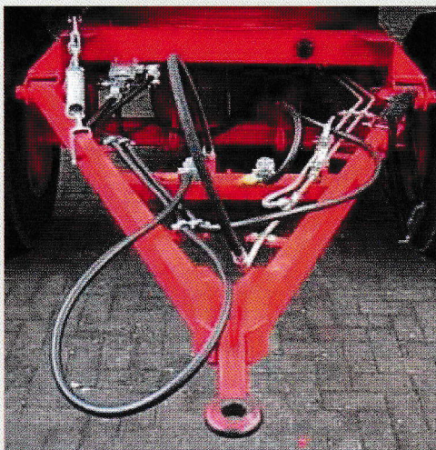
V – drawbar
