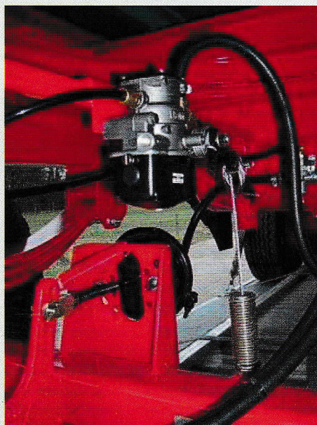
Automatic load depending brake power regulator
