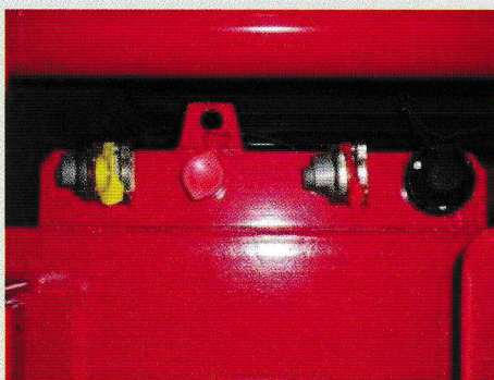
Air / hydraulic / elektrik connection for the 2 nd trailer
