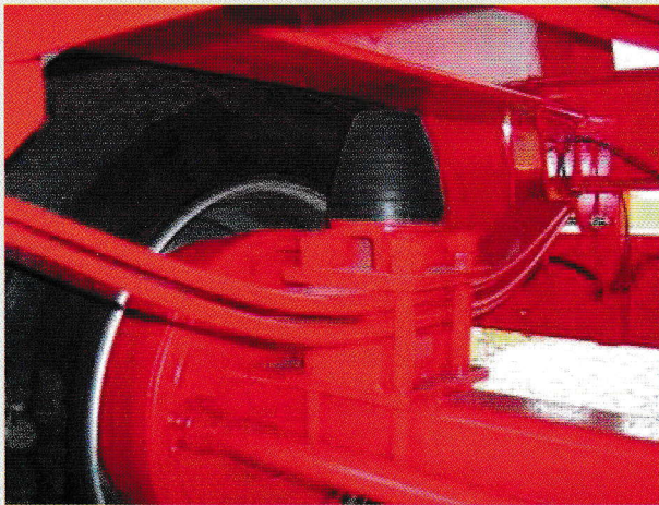
2 sheets and 3 sheets of parable springs with overload insurance
